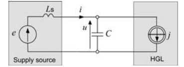
Fig. 17. Equivalent circuit of compensated load for \omega \gg \omega_1
