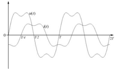
Fig. 6. Voltage and current in a circuit with non-zero distortion power, D
