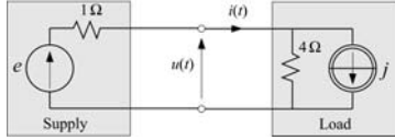
Fig. 11. Circuit with harmonic generating load
